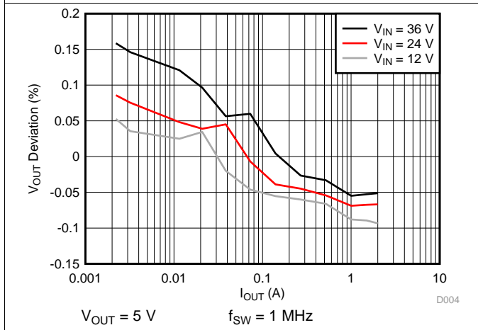
Figure 5. Load Regulation
