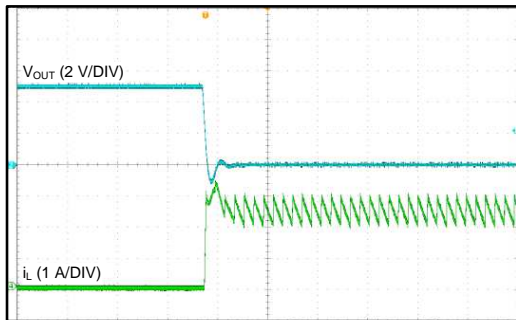
Figure 26. CCM Mode
